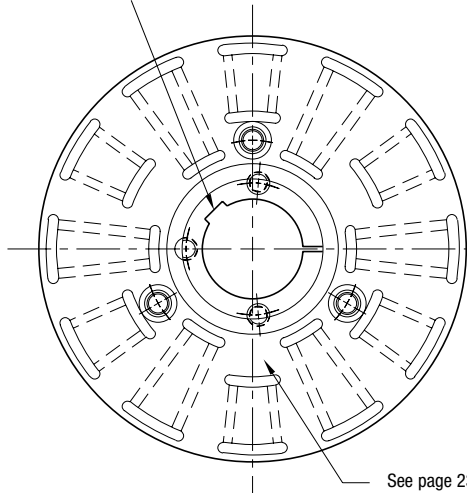
ARMATURE VIEW
