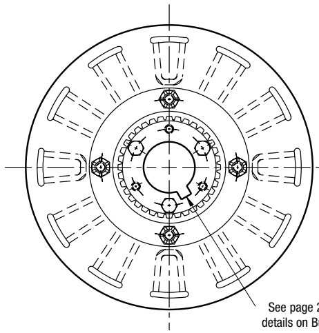
ARMATURE VIEW
