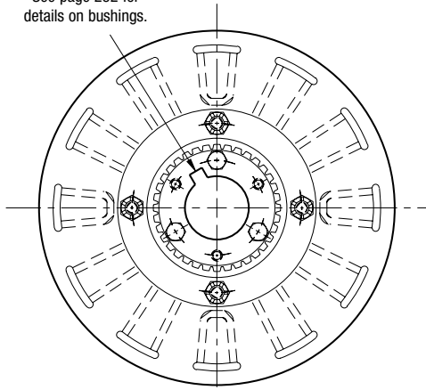
ARMATURE VIEW
