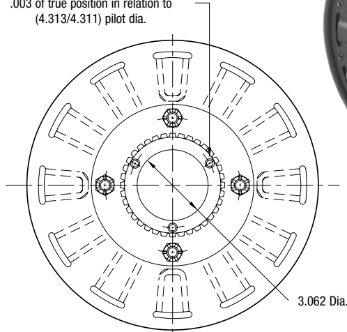
ARMATURE VIEW
