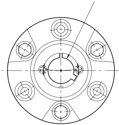
HUB VIEW
