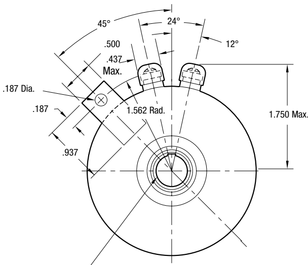
ARMATURE VIEW
